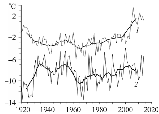
Fig. 1. The temporal variability of average surface air temperature for (1) the warm (April–September) and (2) cold (October–March) seasons and the 11-year moving averages (the heavy lines) for Longyearbyen (Spitsbergen).
