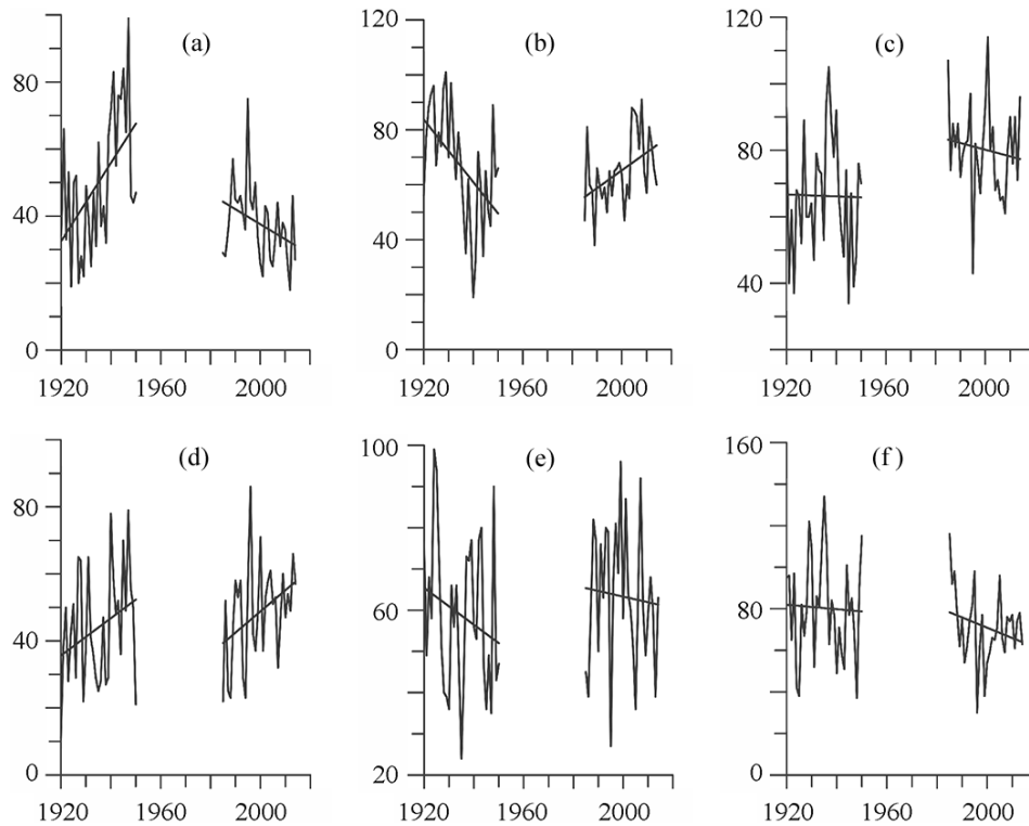
Fig. 2. The temporal variability of the frequency (days) of circulation forms over the periods of the first (1920–1950) and modern (1985–2015) warming for (a, b, c) the cold and (d, e, f) warm seasons. (a, d) C form; (b, e) W form; (c, f) E form.
