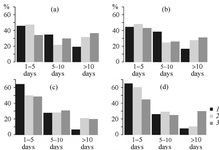
Fig. 3. The frequency (%) of circulation forms revealed during the periods of (a, b) 1920–1950 and (c, d) 1985–2015 for (a, c) the cold and (b, d) warm seasons for the following gradations: short (1–5 days), medium (5–10 days), and long (> 10 days). (1) C form; (2) W form; (3) E form.
